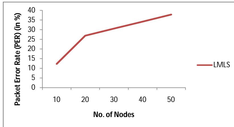
Fig. 3. Packet error rate versus No. of nodes for LMLS
